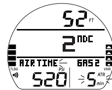
Fig. 43 - NO DECO MAIN (during ATR Alarm)
