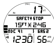
Fig. 50A - SS MAIN (set for Depth/Time prior to dive)
