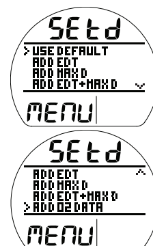
Fig. 34 - SET D MENU (stepping through)
