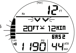
Fig. 57 - DV1 MAIN (during Audible)
