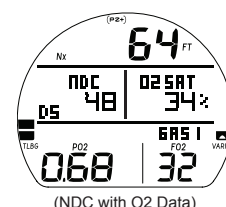
Fig. 44 - NO DECO MAIN (option selected is displayed)
